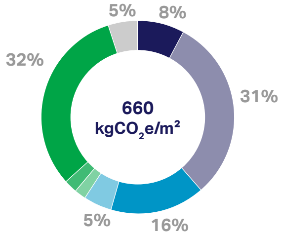
Figure 31: Embodied carbon over the life cycle (A-C)
