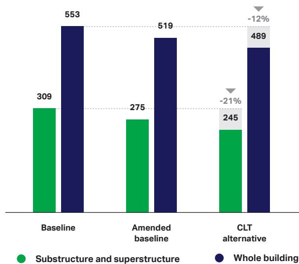
Figure 73: Potential embodied carbon reductions A1-A4 (kgCO 2 e/m 2 GIA)
