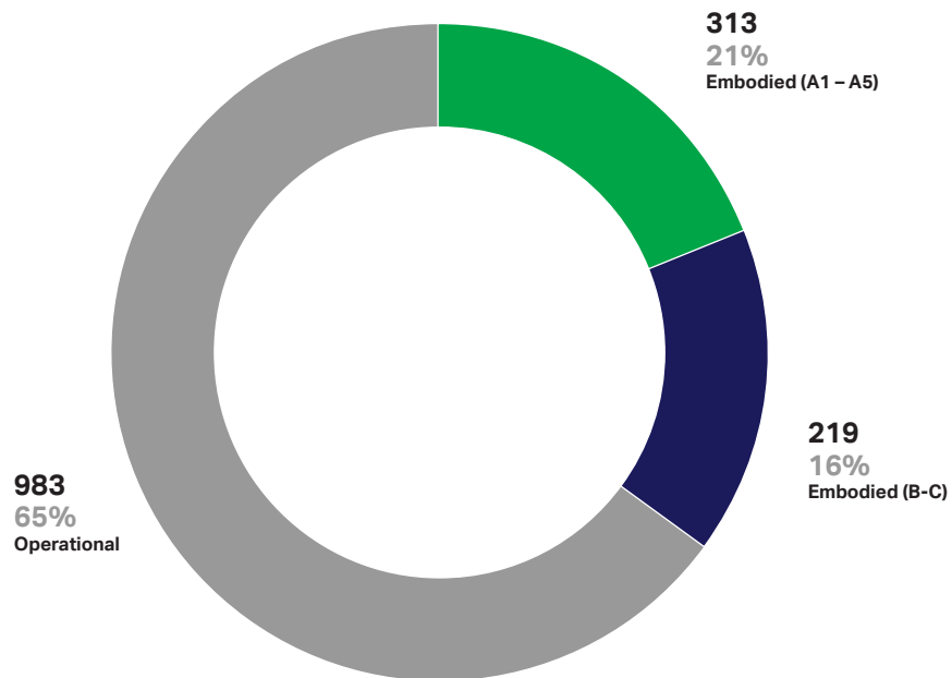
Figure 82: WLCA summary (kgCO 2 e/m 2 )
