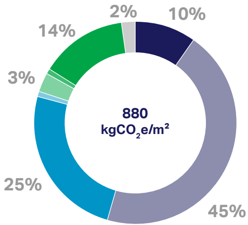
Figure 85: Embodied carbon at practical completion (A1-A5)
