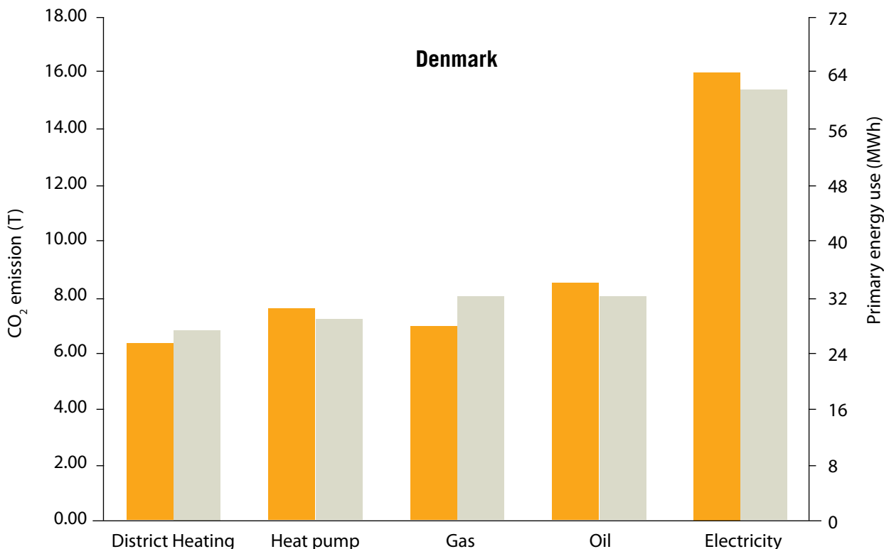
Figure 5: CO 2 emissions and primary energy use for the multi-family house depending on which type of heating energy that is used in the house
