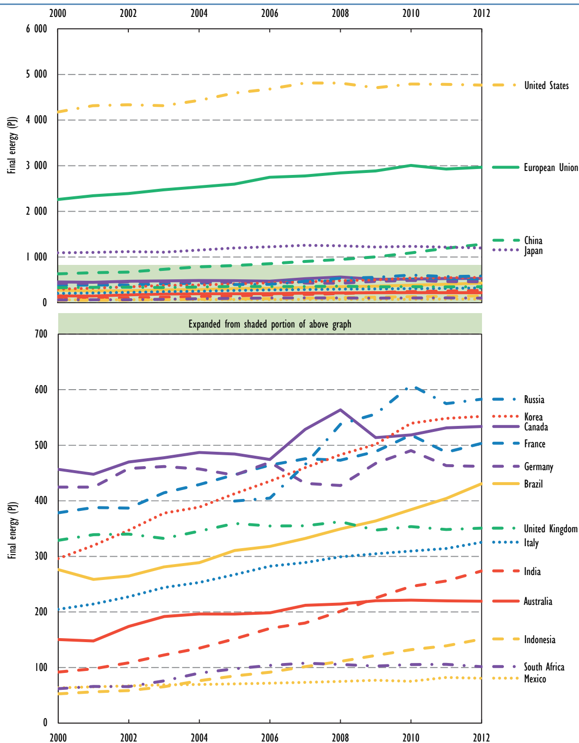
Figure E3 • Services electricity use in MEF economies, 2000-12
