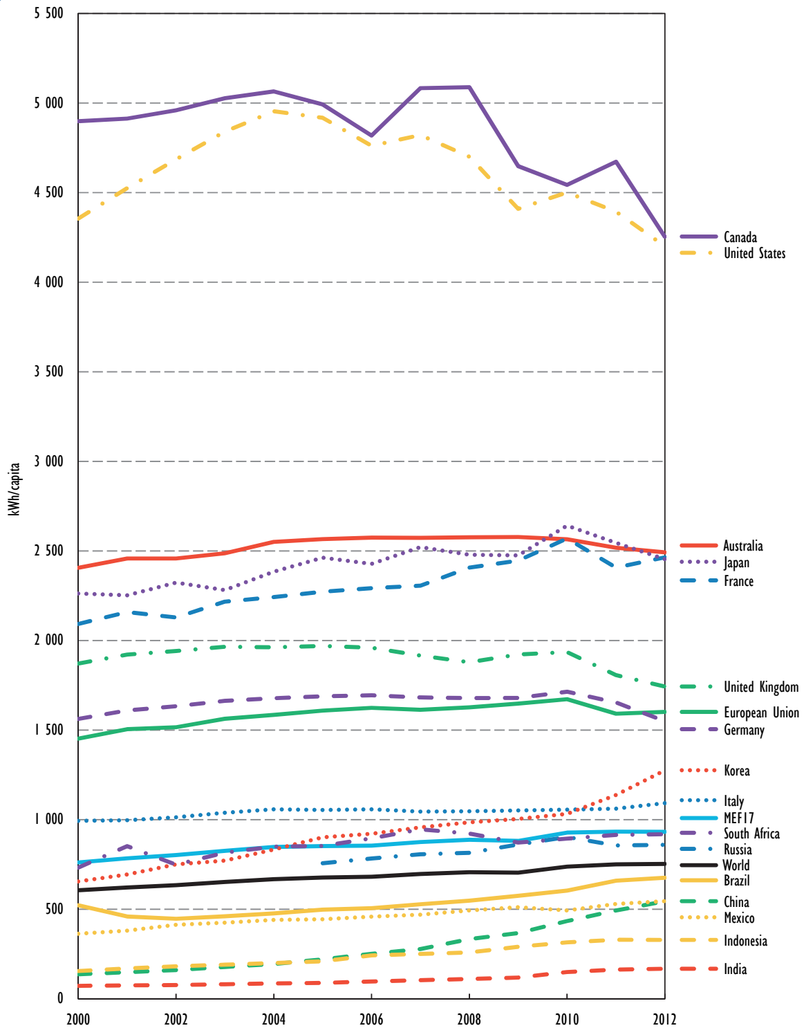
Figure D11 • Residential electricity use per capita in MEF economies, 2000-12
