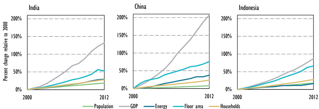
Figure F3 • Change in total building energy use and major drivers in MEF economies, 2000-12
