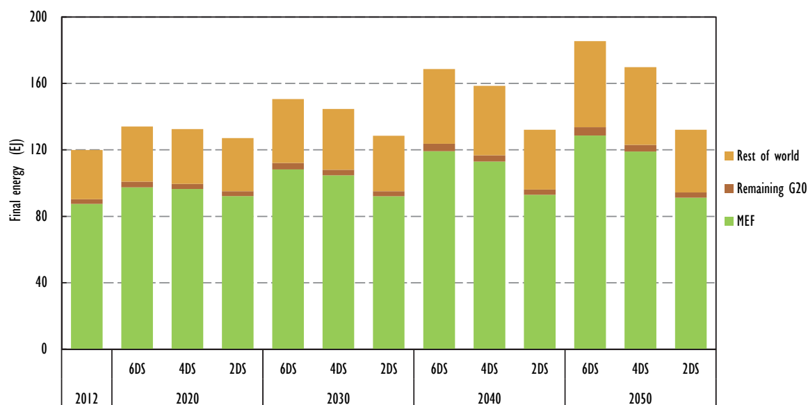
Figure 25 • Building energy scenario forecasts for world, MEF and G20 economies to 2050
