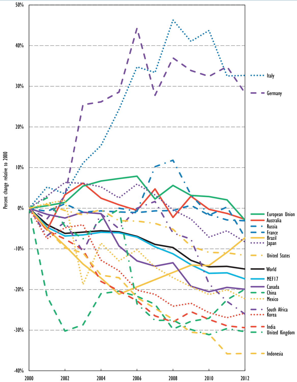
Figure E18 • Change in services energy use per floor area in MEF economies, 2000-12
