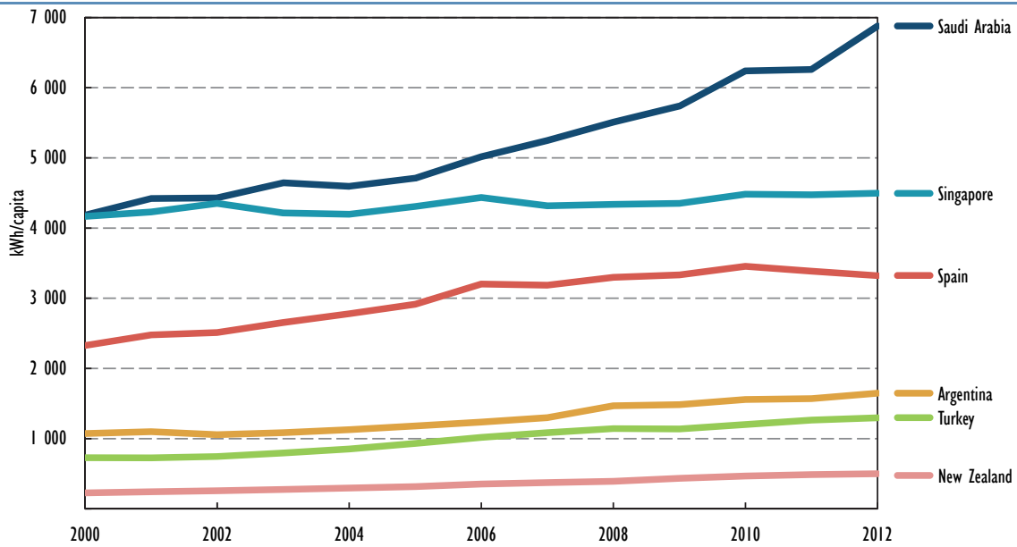
Figure 23 • Building electricity use per capita in G20 and guest economies, 2000-12
