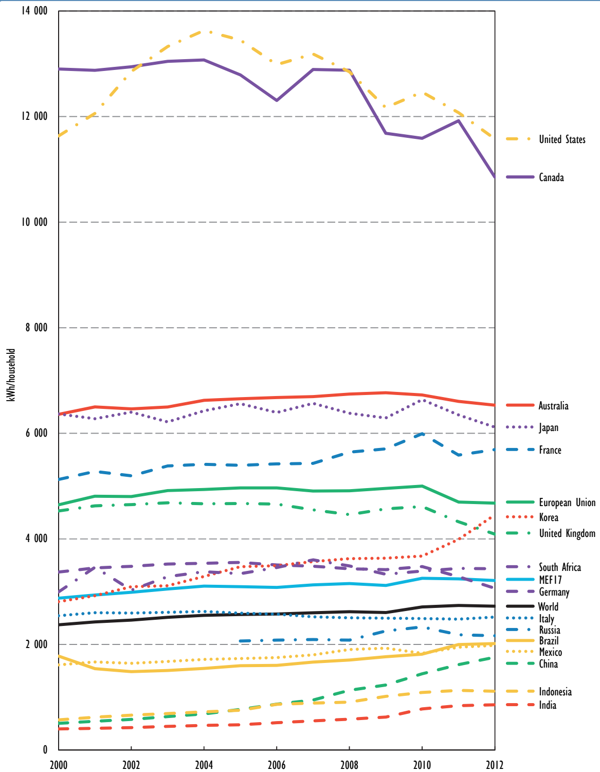
Figure D23 • Residential electricity use per household in MEF economies, 2000-12
