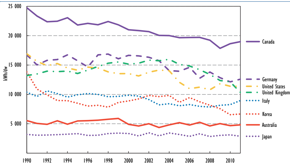
Figure C1 • Residential space-heating energy use per dwelling
