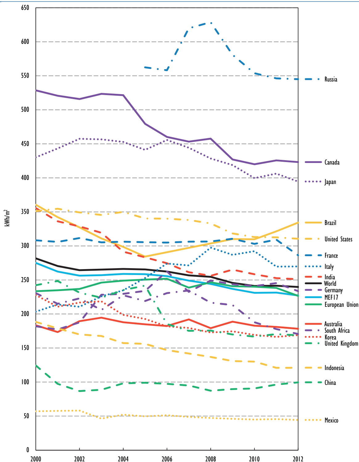
Figure E17 • Services energy use per floor area in MEF economies, 2000-12
