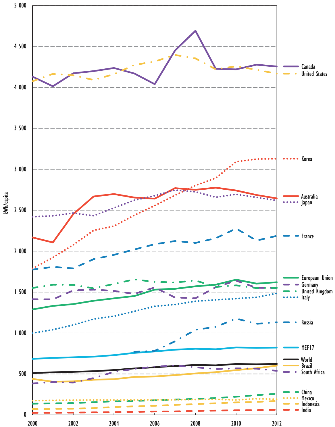
Figure E11 • Services electricity use per capita in MEF economies, 2000-12
