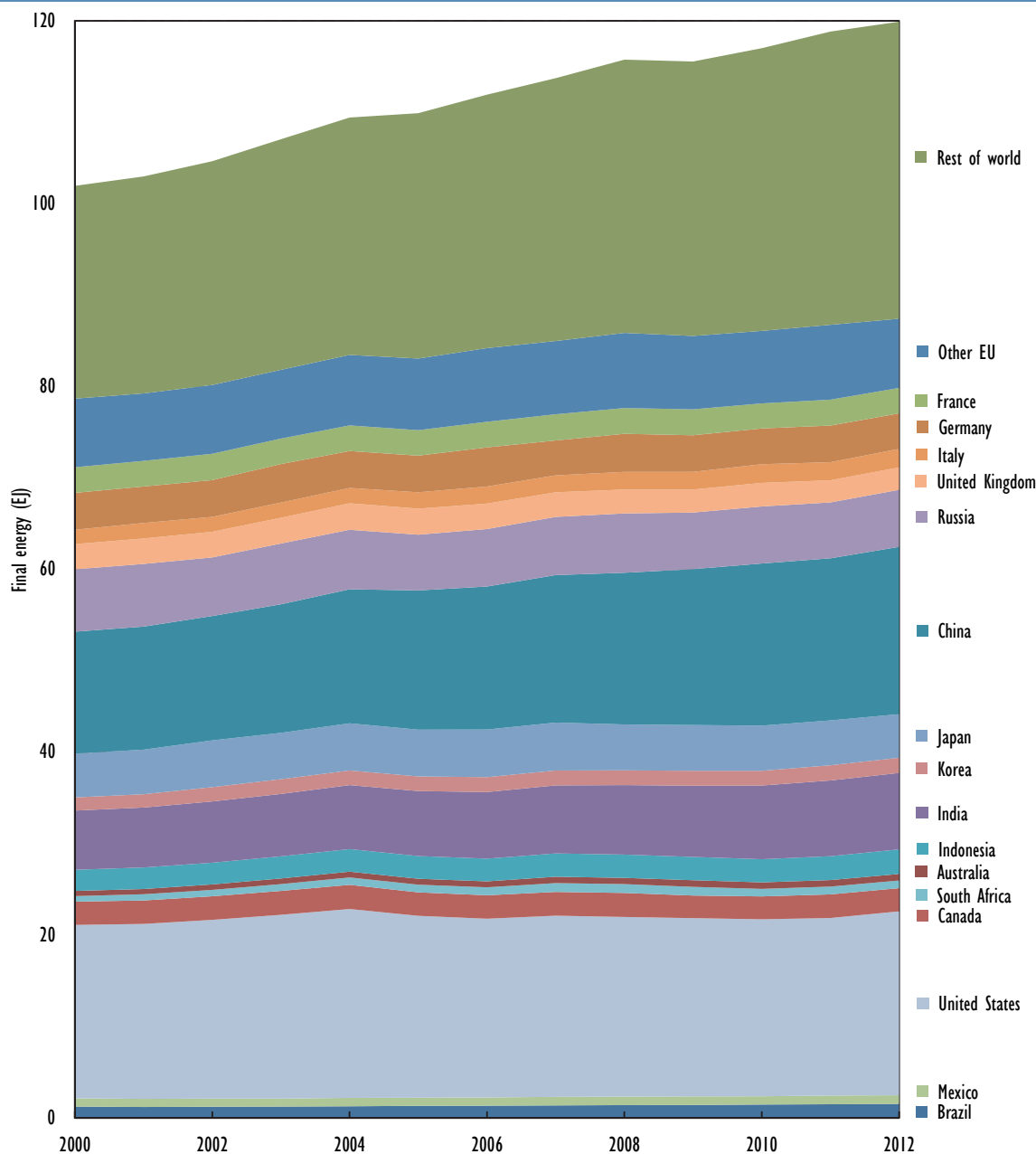
Figure 1 • Total building energy use in MEF economies and the world, 2000-12
