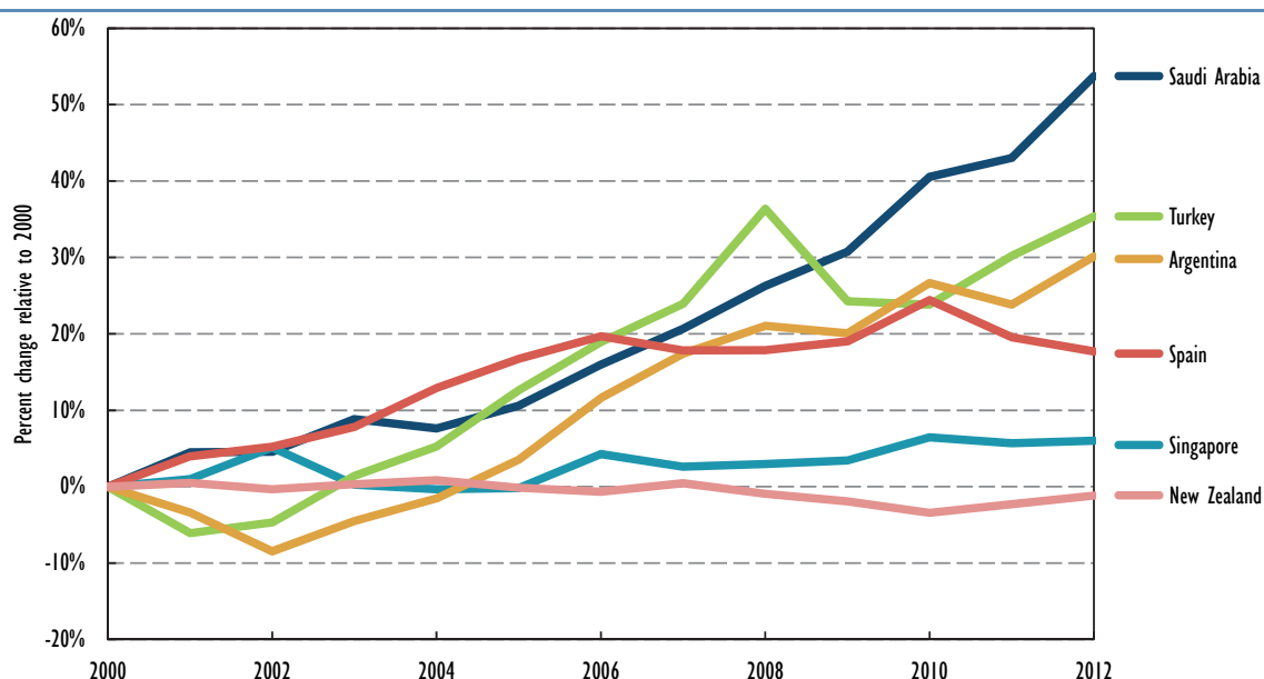
Figure 22 • Change in building energy use per capita in G20 and guest economies, 2000-12
