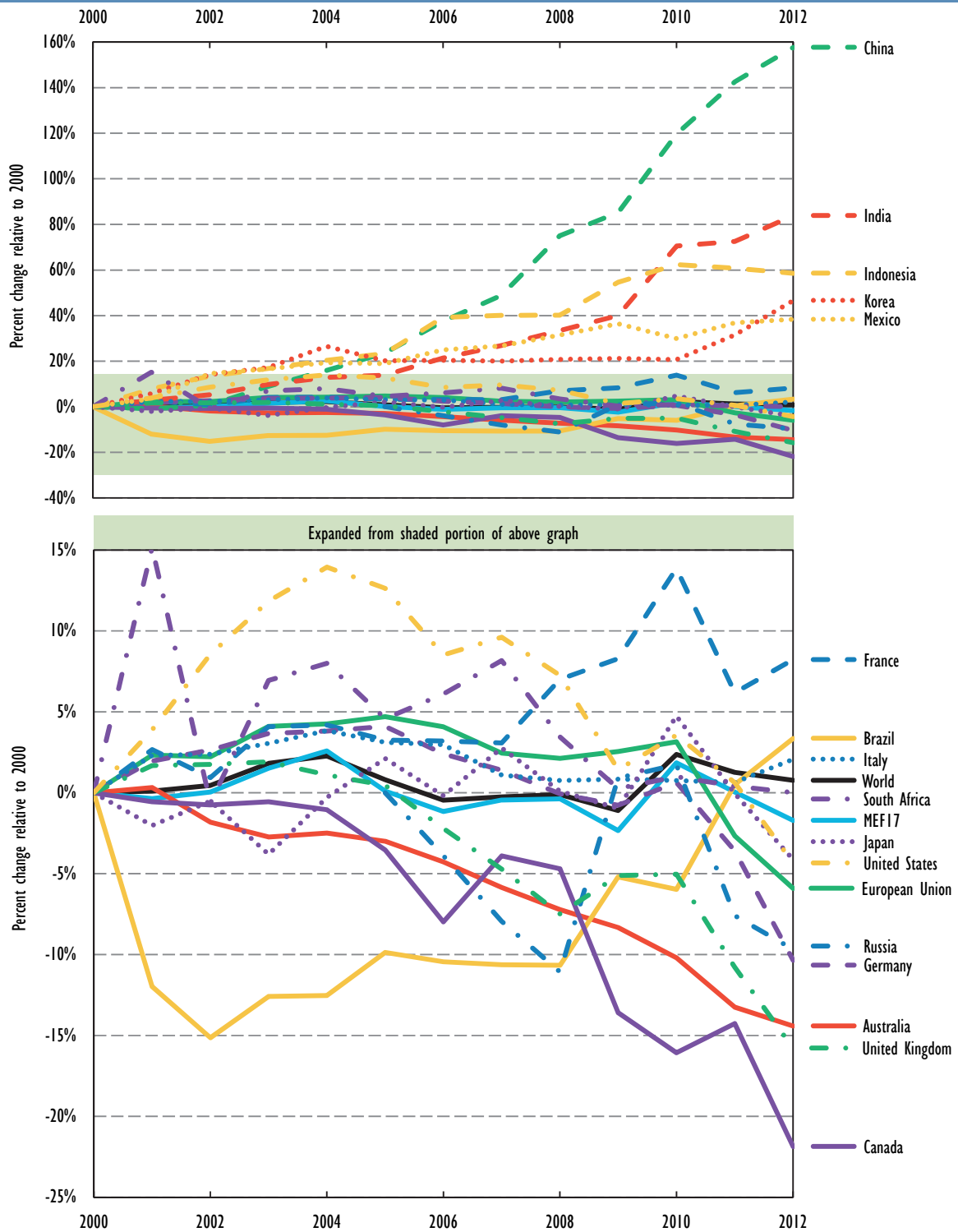
Figure D20 • Change in residential electricity use per floor area in MEF economies, 2000-12
