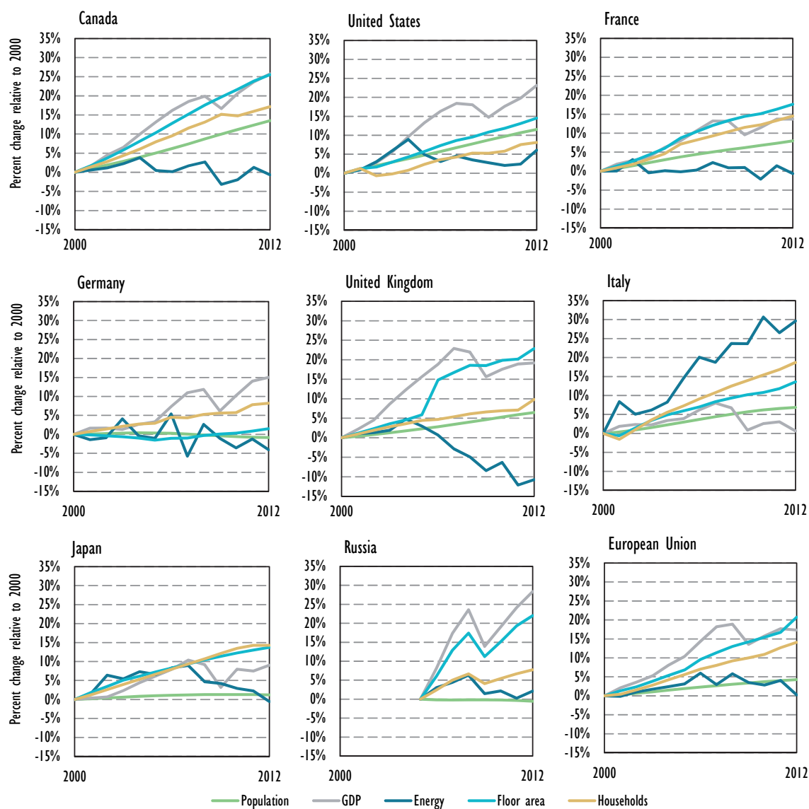
Figure F1 • Change in total building energy use and major drivers in MEF economies, 2000-12
