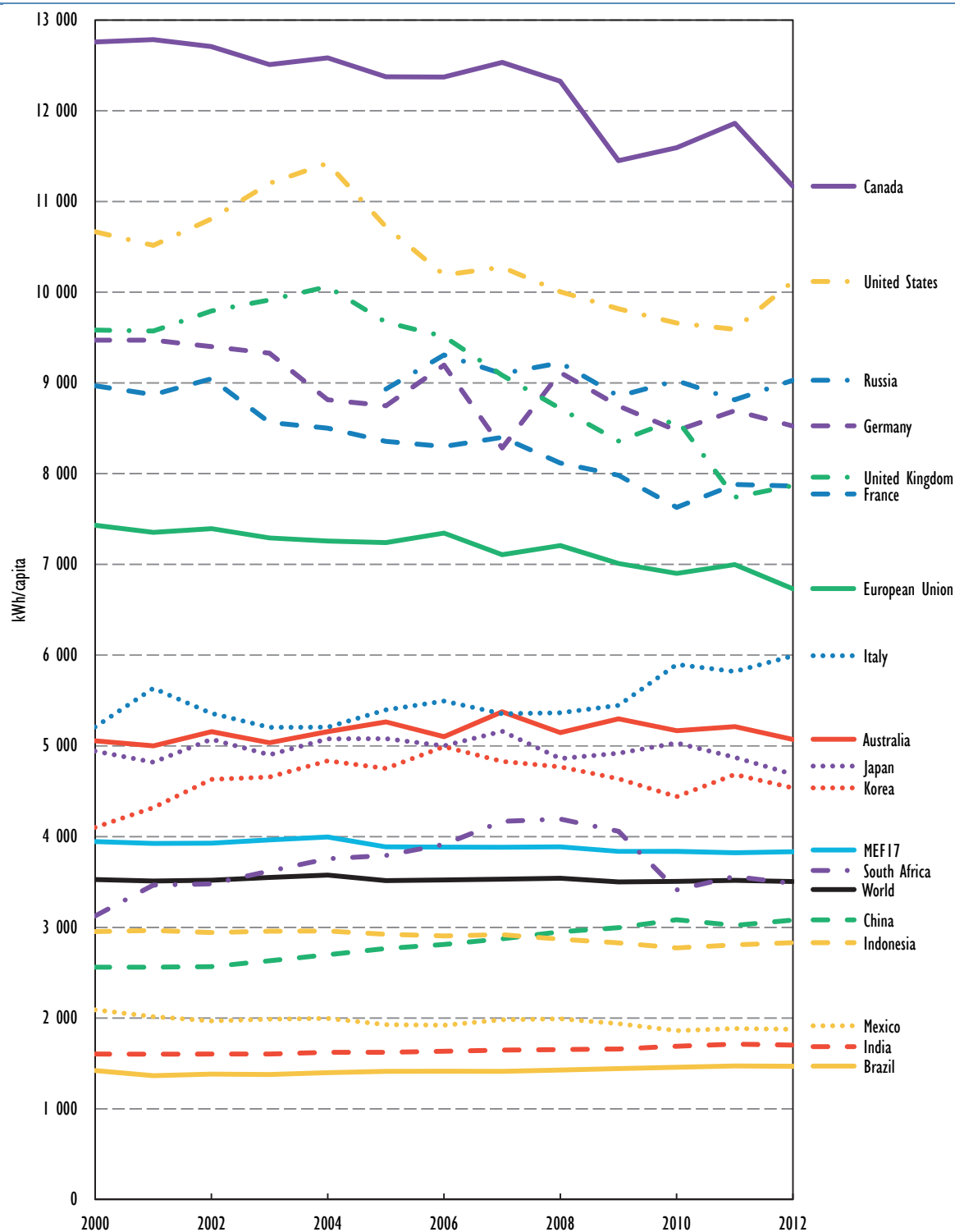
Figure D9 • Residential energy use per capita in MEF economies, 2000-12
