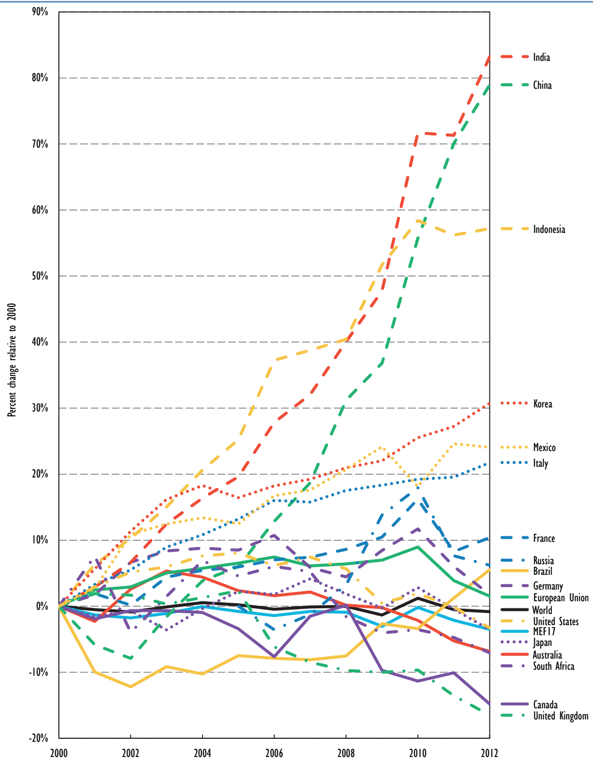
Figure 16 • Change in building electricity use per floor area in MEF economies, 2000-12
