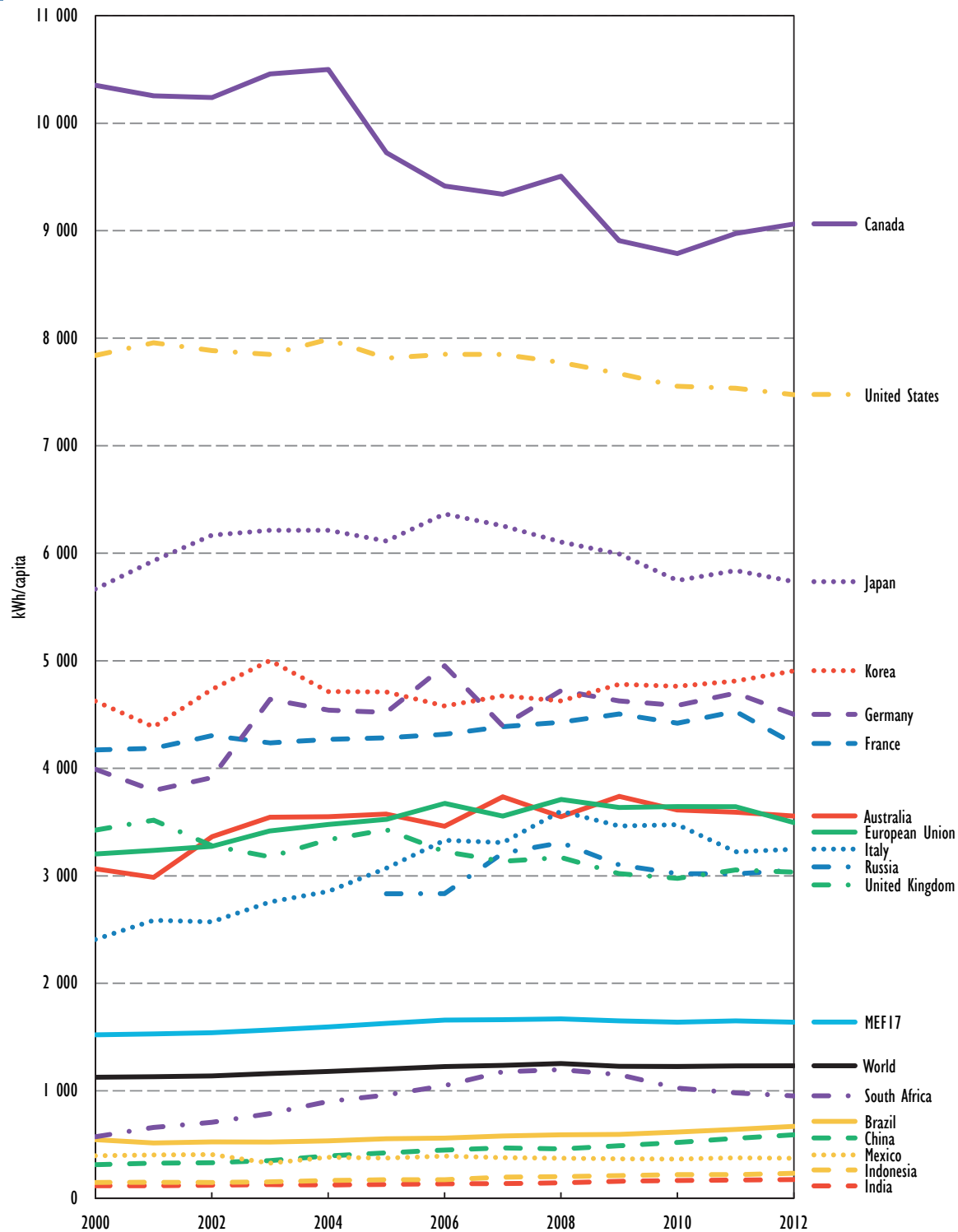
Figure E9 • Services energy use per capita in MEF economies, 2000-12
