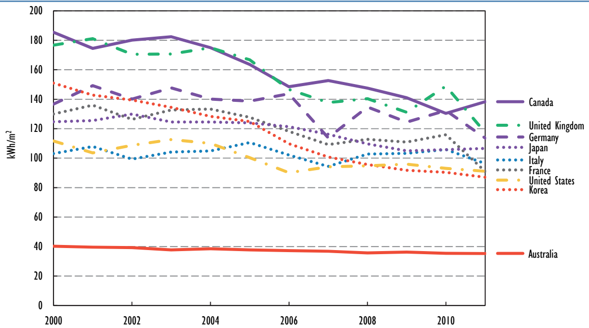
Figure C5 • Residential fossil fuel energy use per floor area
