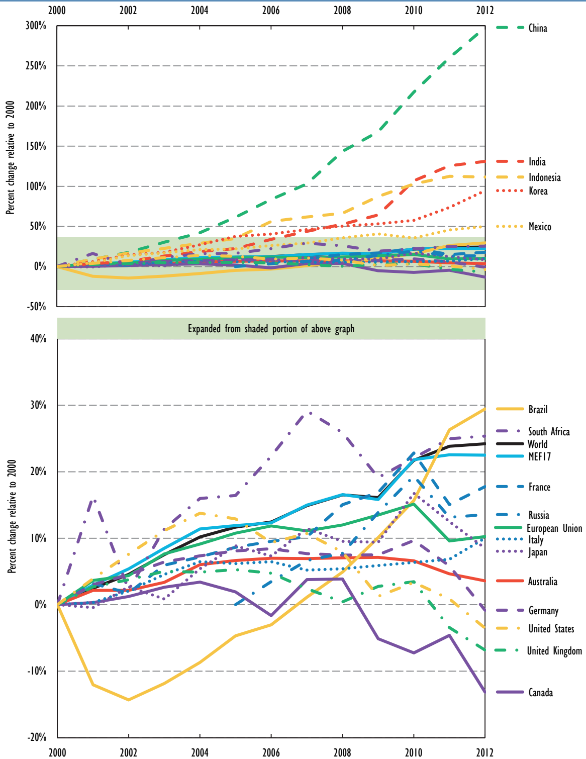
Figure D12 • Change in residential electricity use per capita in MEF economies, 2000-12
