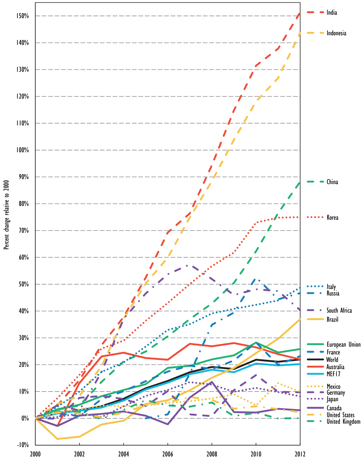
Figure E12 • Change in services electricity use per capita in MEF economies, 2000-12
