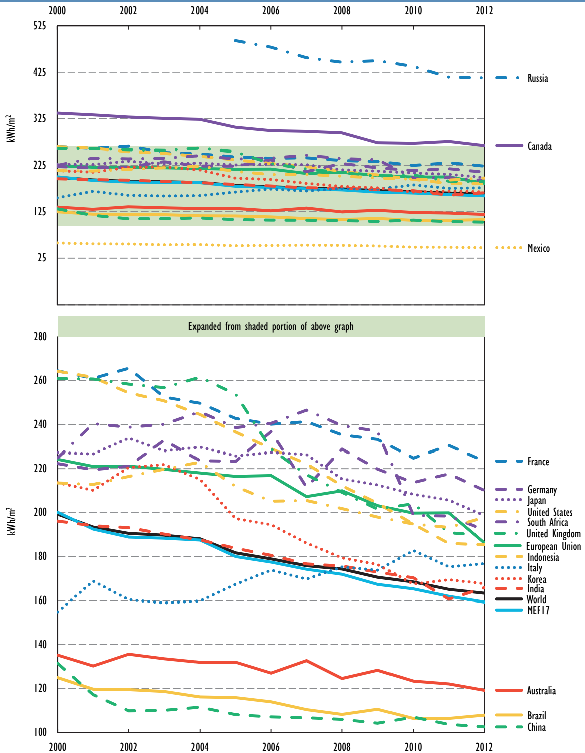
Figure 13 • Building energy use per floor area in MEF economies, 2000-12
