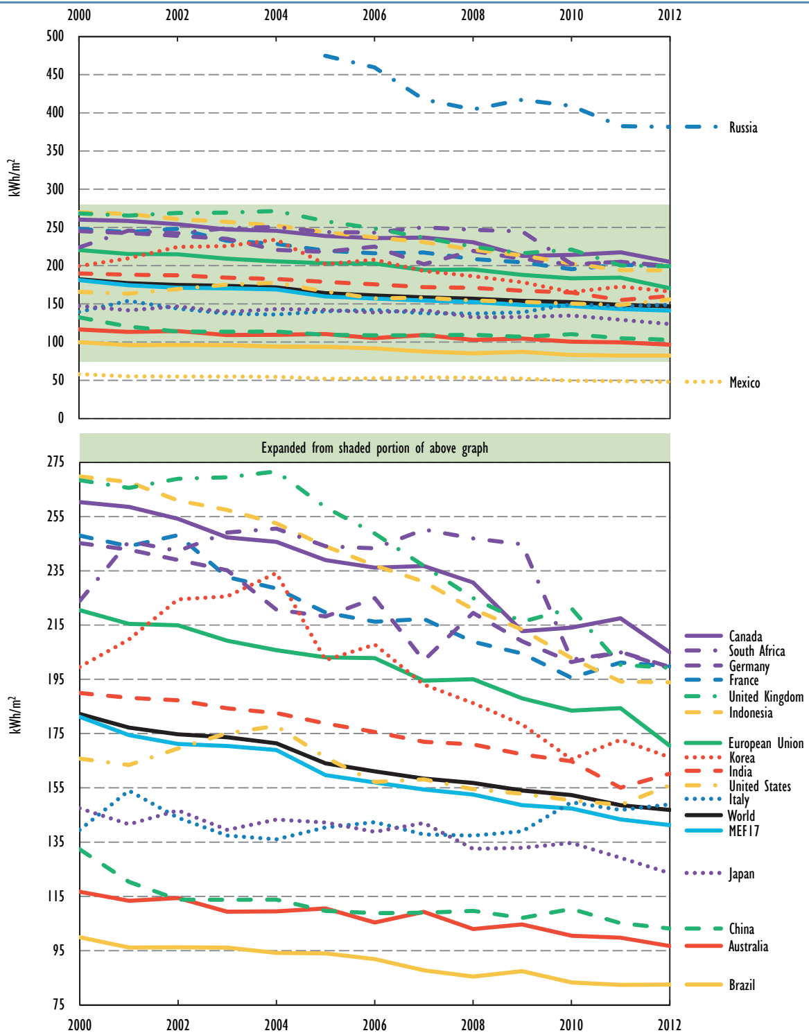
Figure D17 • Residential energy use per floor area in MEF economies, 2000-12
