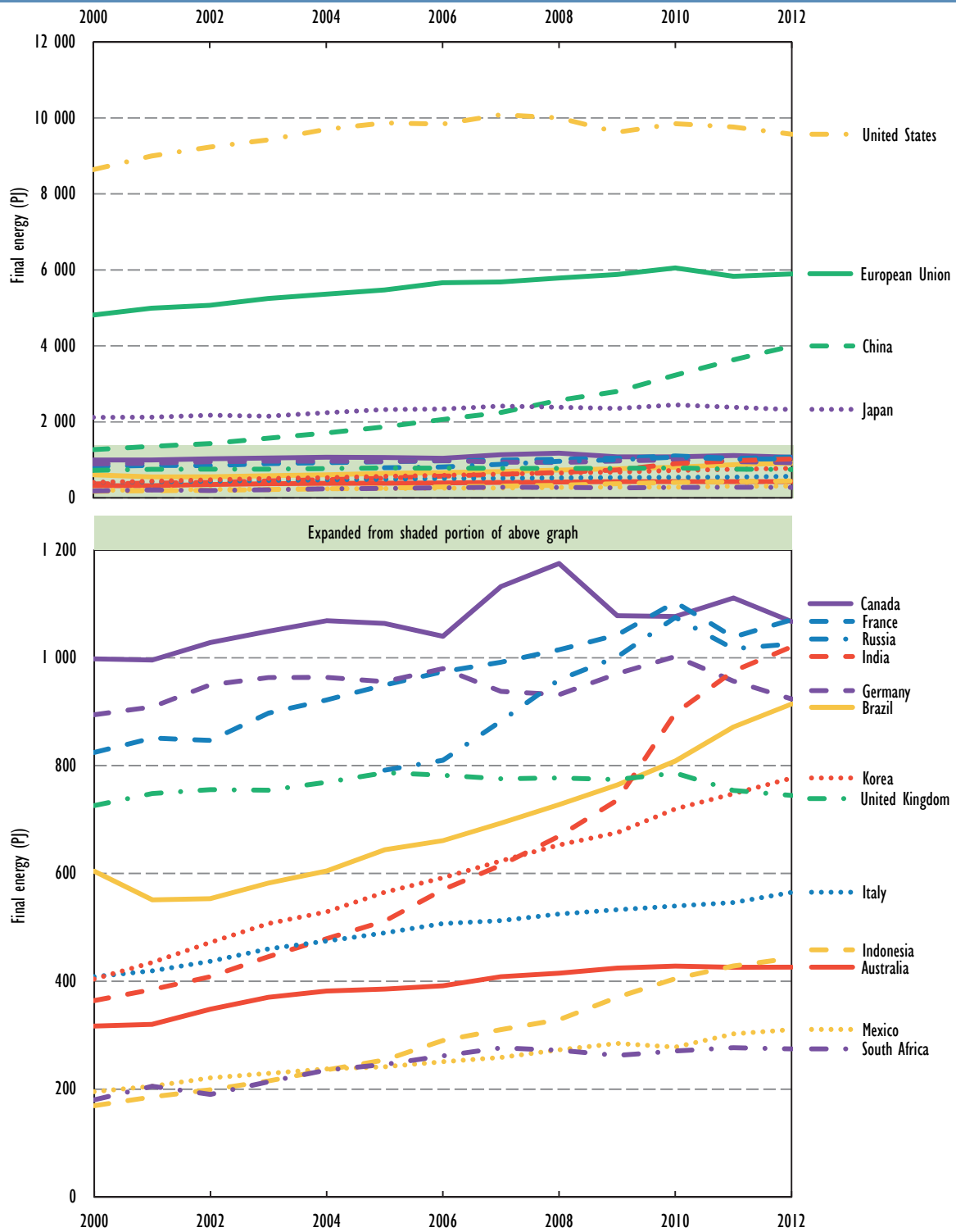
Figure 7 • Building electricity use in MEF economies, 2000-12
