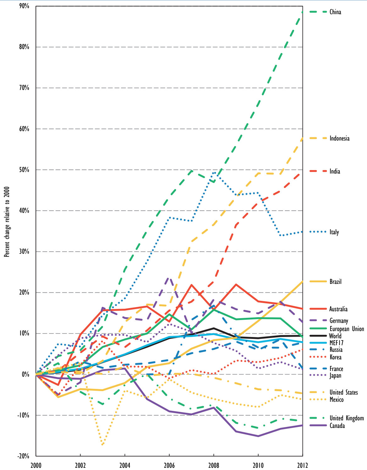
Figure E10 • Change in services energy use per capita in MEF economies, 2000-12
