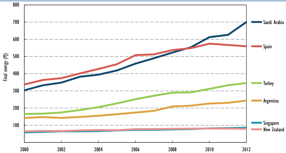
Figure 19 • Building electricity use in G20 and guest economies, 2000-12
