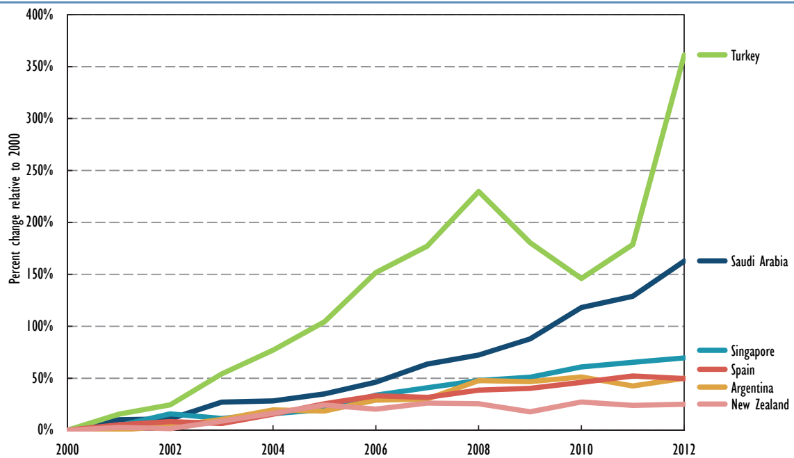
Figure E6 • Change in services energy use in G20 and guest economies, 2000-12
