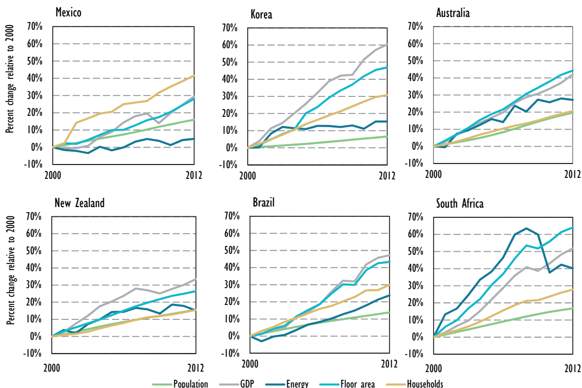
Figure F2 • Change in total building energy use and major drivers in MEF economies, 2000-12
