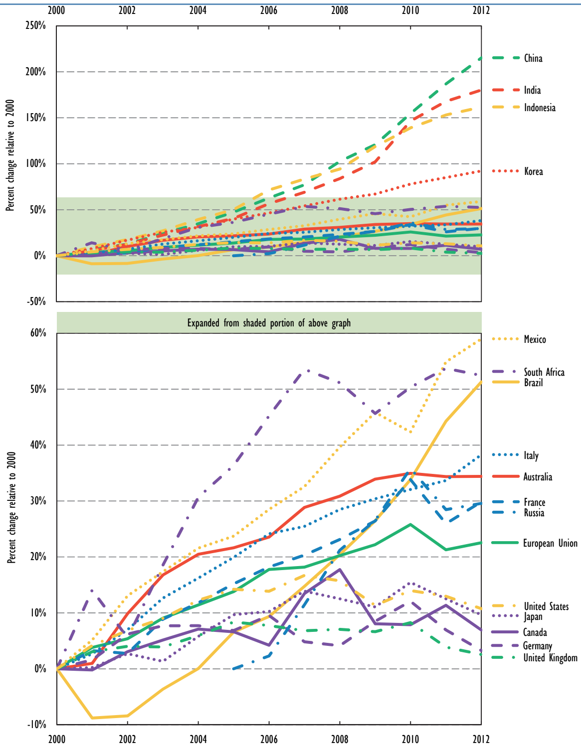
Figure 8 • Change in building electricity use in MEF economies, 2000-12
