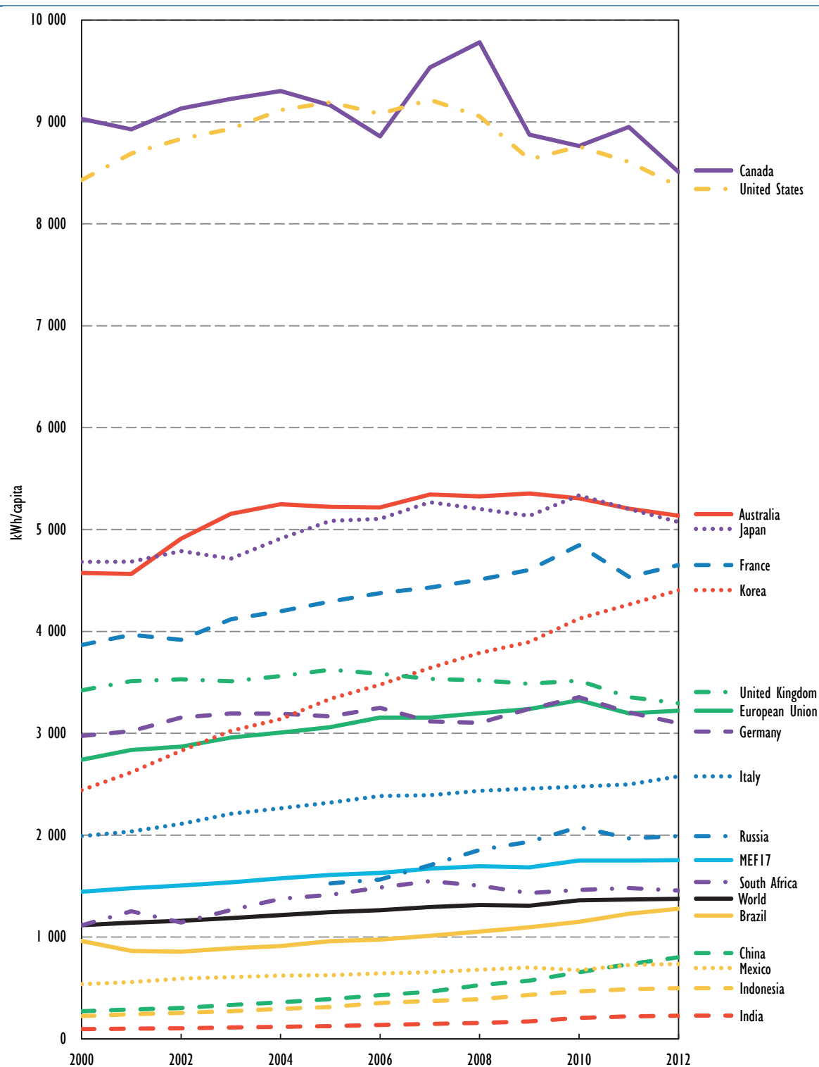
Figure 11 • Building electricity use per capita in MEF economies, 2000-12
