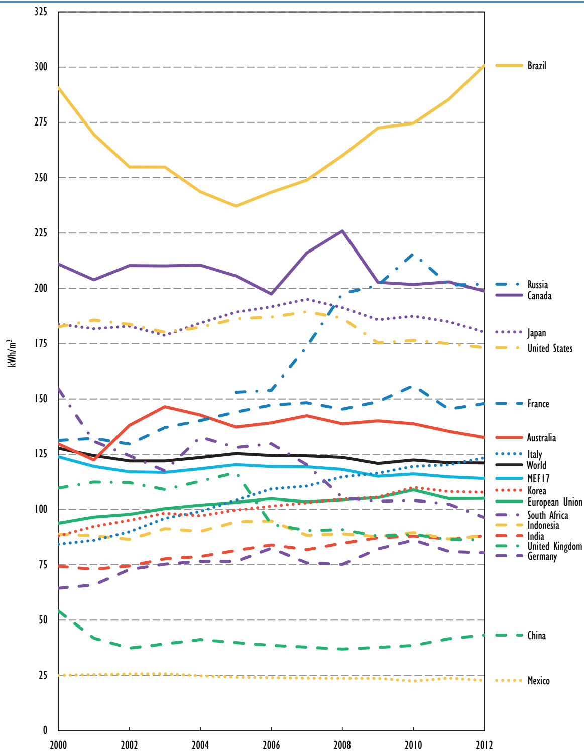
Figure E19 • Services electricity use per floor area in MEF economies, 2000-12
